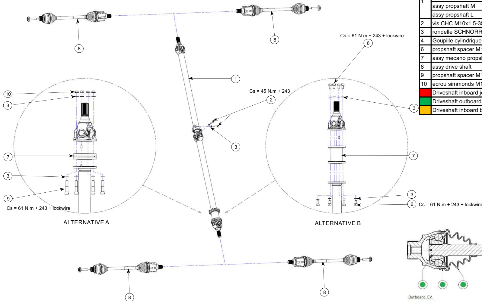
Outboard CV Grease MS9U024 Total grease volume 150g ± 5g
