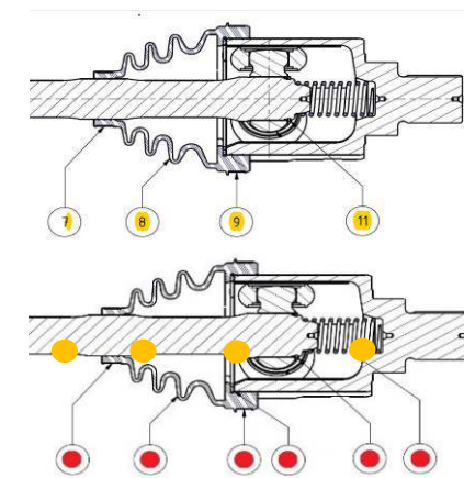
Inboard Joint Grease MS9U025 (XP595) Volume 165g +/- 5g
