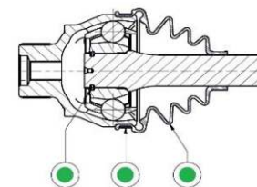
Outboard CV Grease MS9U024 Total grease volume 150g ± 5g
